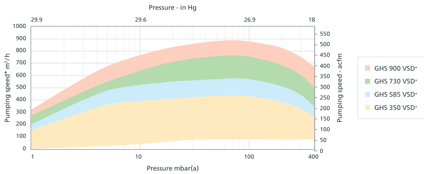
*Pumping speed at element inlet at steady state - according ISO 21360-1:2012 (E).
